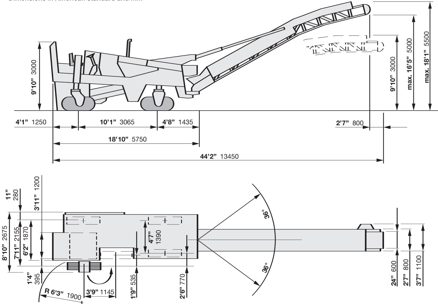
Cold milling machine W 1200 F on crawler tracks Dimensions in American standard and mm
