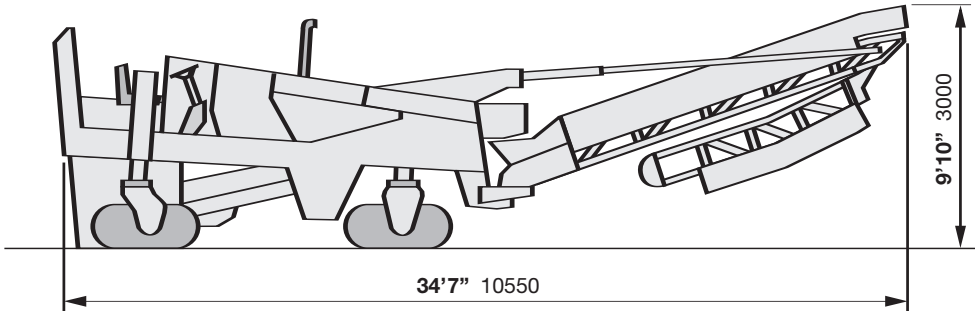
Special equipment: Folding discharge conveyor Dimensions in American standard and mm
